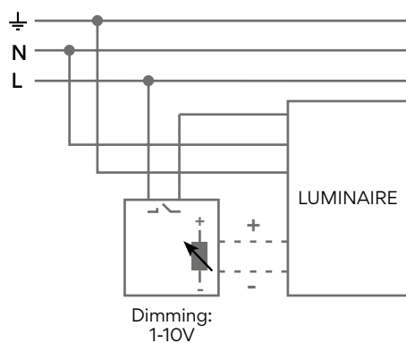
2 1-10V System control
