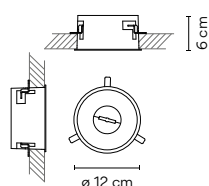
Built-in Canopy E3 Ø 120 mm.
