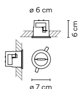
Remote Built-in Canopy E4 Ø 60 mm.
