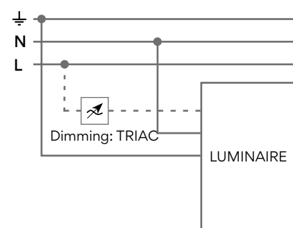
6 TRIAC control
