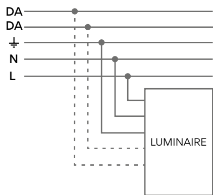
3 DALI System control
