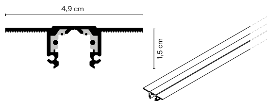
T011 11/OM Trimless track 1 m T012 11/OM Trimless track 2 m T013 11/OM Trimless track 3 m
