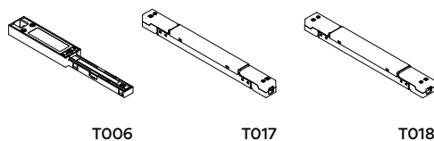
T010 11/OM Electrical connection 100W surface T006 11/OM Remote feeder for surface track (Required with T017 and T018) T017 80/OM Electrical connection 48W remote T018 80/OM Electrical connection 84W remote
