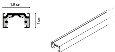
T001 11/OM Surface track 1 m T002 11/OM Surface track 2 m T003 11/OM Surface track 3 m
