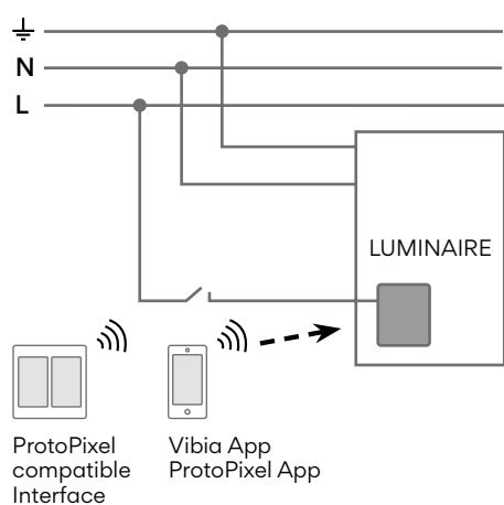
5 ProtoPixel control
